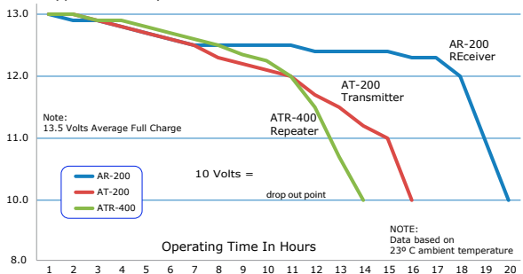
Typical Battery Life for BA-5390/U
